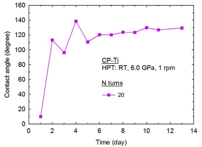
Fig. 7. Variation of contact angle of 20 turns samples with observation period.
