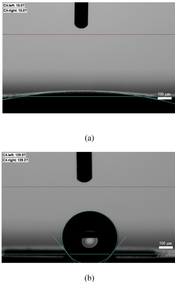
Fig. 8. Contact angle images for 20 turns samples with different observation periods: (a) 1 day, (b) 13 days.
